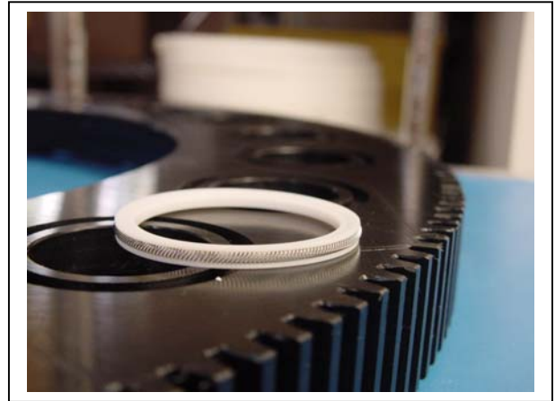
Figure 2-11: Variseal® Installation
