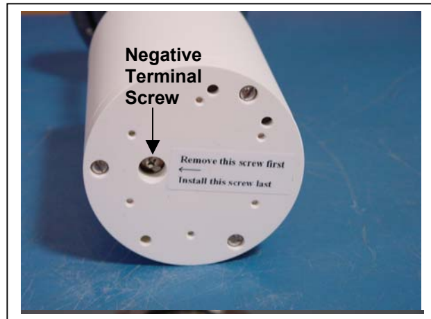
Figure 4-8: Battery End Cap
